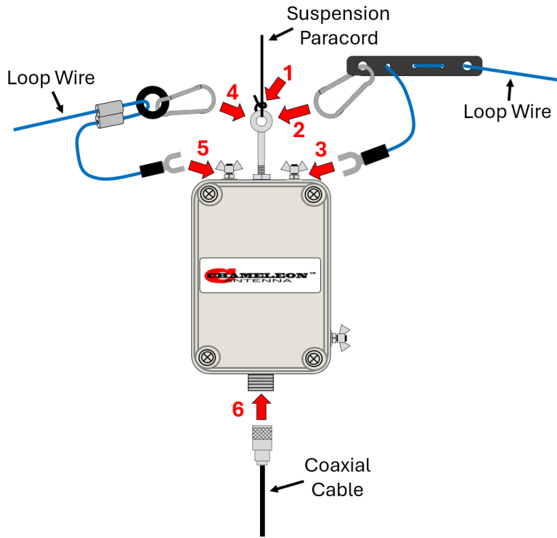
Connection Detail
