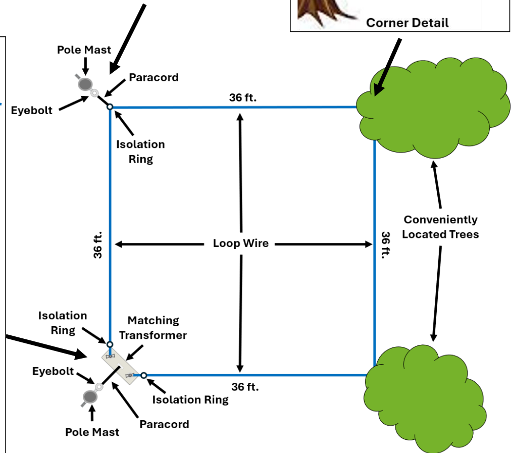
Notional SKYLOOP 40 Installation
